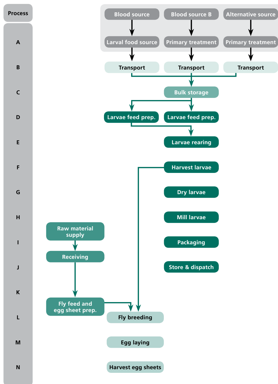
FIGURE 9.1 Agriprotein fly protein production process
